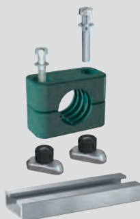
Installation with mounting rail
